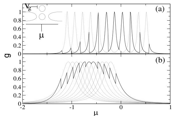
FIG. 1. Conductance (solid line) through one connected state with ten disconnected states as function of chemical potential. (a) Intermediate coupling case: \epsilon = -1.08 , t = 0.2 , U = 0.16 , and e_m = -1.2 + 0.02m ( m = 1, \dots, 10 ). (b) Strongly connected case: \epsilon = -1 , t = 0.5 , U = 0.08 , e_m = -1.24 + 0.04m . Dotted curves: Conductances for fixed occupations n_d = 0, \dots, 10 of the disconnected states. As n_d changes with \mu , the conductance (solid line) switches accordingly. Inset: Schematic of the connected and disconnected dots.
