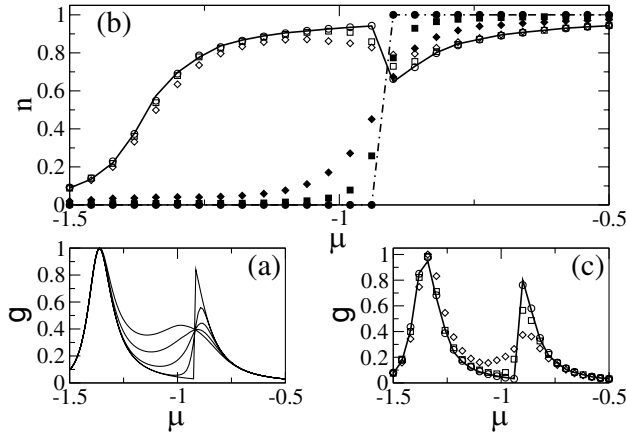
FIG. 3. (a) Temperature dependence of the conductance as function of \mu (connected state: \epsilon = -1.3 ; disconnected state: e_1 = -1.26 ; U = 0.4 ; t = 0.3 ). The different curves correspond to \pi kT = 0, 0.1, 0.2, 0.3, 0.4 . (b) Occupation of the connected state n_\alpha (open symbols) and disconnected state n_d (filled symbols) for several values of couplings as the disconnected state opens up additional non-current-carrying lead. Lines: results of the exact solution of Eq. (3); symbols: DMRG calculations for different couplings of the disconnected state (circles t = 0 , squares t = 0.1 , diamonds t = 0.2 ). (c) Conductance of connected state in (b).
