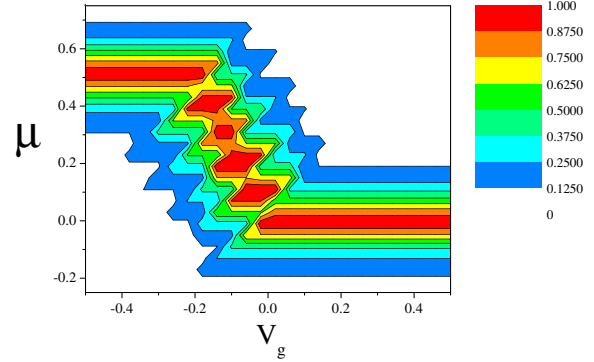
FIG. 2 (color online). Conductance as a function of overall chemical potential \mu and external gate voltage V_g for the disconnected states (see inset in Fig. 1). Connected state: \epsilon = 0 ; disconnected states: e_m = -0.55 + 0.05m ( m = 1, \dots, 5 ), U = 0.1 , and t = 0.2 .
