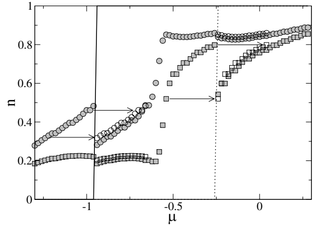
FIG. 4. Occupation for two connected states ( t = 0.5 ) at \epsilon_1 = -1.1 (gray circles) and \epsilon_2 = -1 (gray squares) and two disconnected states e_1 = -1.12 (solid line), e_2 = -1.02 (dotted line) as function of \mu obtained from DMRG ( U = 0.3 ). To demonstrate that right after the switch n_\alpha(\mu) = n_\alpha(\mu - U) , we plot n_\alpha(\mu + U) for values of \mu prior to the switch, i.e., -1.2 < \mu < -1 and -0.48 < \mu < -0.28 (white symbols). A clear overlap between the white and gray symbols is seen.
