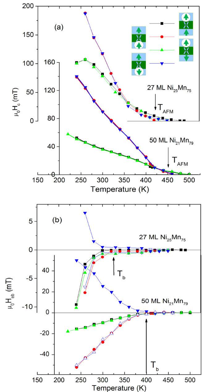
Figure 3. Temperature dependence of coercivity (a) and exchange-bias field (b) for \sim 25 ML Ni/ \sim 50 ML Ni 21 Mn 79 /12.9 ML Ni/Cu 3 Au(001) and 22 ML Ni/27 ML Ni 25 Mn 75 /11.9 ML Ni/Cu 3 Au(001), measured with polar MOKE. The different spin configurations of the FM layers at the upper and lower interface are symbolically shown in front of the corresponding legend. The antiferromagnetic ordering temperature T_{AFM} and blocking temperature T_b are indicated in both figures by arrows. Open blue symbols in (b) represent a mirror of the same-color filled symbols with positive EB.
