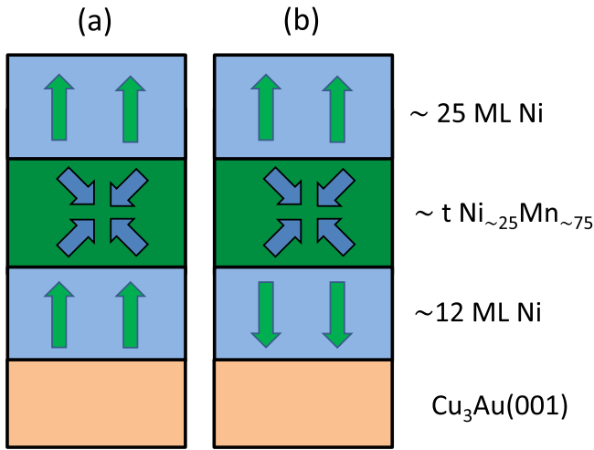
Figure 1. Schematic illustration of the two prepared samples of the FM2/AFM/FM1 trilayer system when the magnetizations of the two FM layers are (a) parallelly and (b) antiparallelly aligned. The approximate thicknesses of FM1, FM2, and AFM, as well as the approximate composition of the latter are shown, where t stands for \sim 27 or \sim 50 ML thickness of \text{Ni}_{\sim 25}\text{Mn}_{\sim 75} .
