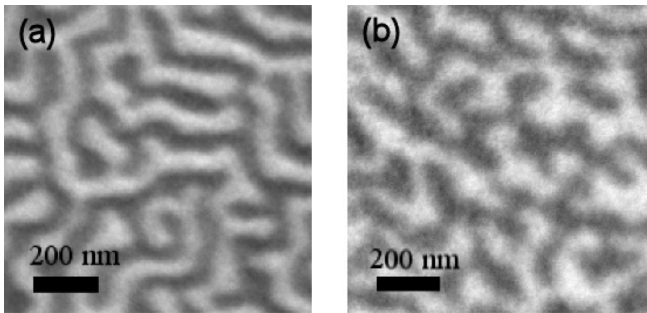
FIG. 1. XMCD-PEEM images of 1 \mu\text{m} \times 1 \mu\text{m} area of the room temperature demagnetized domain state of (a) L1_0 -ordered FePd and (b) FePt films in zero magnetic field. Dark and bright areas depict magnetic domains of oppositely orientated magnetization perpendicular to the film plane.
