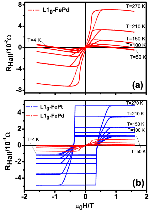
FIG. 2 (color online). Measured Hall resistance R_{\text{Hall}} for various temperatures ranging between T = 4 and 270 K for (a) L1_0 -FePd and (b) L1_0 -FePt epilayers. The measured AHE signal is, for all temperatures, much larger in L1_0 FePt as compared to L1_0 FePd, as shown in (b).
