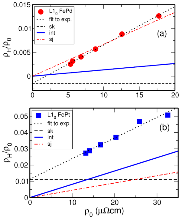
FIG. 3 (color online). Resistivity ratio of measured transverse and longitudinal resistivity \rho_H/\rho_0 versus longitudinal resistivity \rho_0 for (a) L1_0 FePd (circles) and (b) L1_0 FePt (squares). The thin black dotted line is a linear \Phi_{\text{sk}} + \kappa\rho_0 fit to the measured ratio yielding \Phi_{\text{sk}} (dashed line) and \kappa . The intrinsic contribution \kappa^{\text{int}}\rho_0 (solid thick line) calculated from first principles as well as the side-jump contribution (\kappa - \kappa^{\text{int}})\rho_0 = \kappa^{\text{sj}}\rho_0 (dot-dashed line) yield a linear dependence in \rho_H/\rho_0 versus \rho_0 (see also Table II). The total \rho_H/\rho_0 signal is a sum of skew scattering \Phi_{\text{sk}} and intrinsic plus side-jump contributions.
