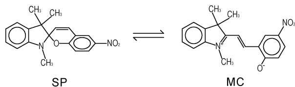
Figure 1. Structure of 1,3,3-trimethylindolino-6-nitrobenzopyrrolospiran (SP) and one of its merocyanine (MC) zwitterionic isomers. While SP is chiral and possesses two halves with orthogonal planes, the conjugated MC form is planar and prochiral. At the metal surface, each of the four different conformations of the MC isomer (given by combinations of the two possible rotations of both the phenolate and indole groups) is expected to appear indistinctly under its two chiral forms.
