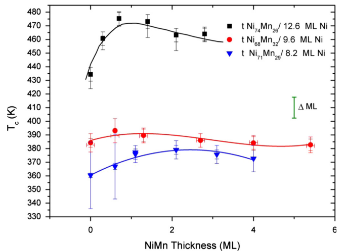
Fig. 3. Ni Curie temperature as a function of the Ni x Mn 1-x thickness at different Ni concentrations in the Ni-rich regime. The scale bar at the right indicates the difference in Curie temperature corresponding to a 1 ML change of the effective Ni thickness estimated from the linear fit in Fig. 2.
