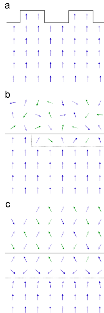
Fig. 6. Schematic model for the Ni Curie temperature changes as a function of the Ni x Mn 1-x thickness in the Mn-rich regime. (a) Ni layer, (b) thin layer of Ni x Mn 1-x on top, and (c) thicker layer of Ni x Mn 1-x with antiferromagnetic order.
