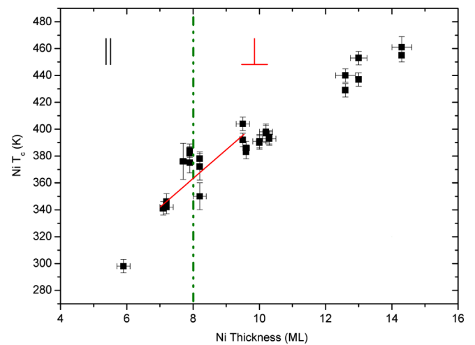
Fig. 2. Curie temperatures of Ni/Cu 3 Au (001) as a function of Ni thickness. The vertical dashed line marks the SRT around 8 ML Ni thickness. The straight line is a linear fit from 7 ML to 10 ML used to correlate the Curie temperature variation in NiMn/Ni bilayers to a change of the effective Ni thickness.
