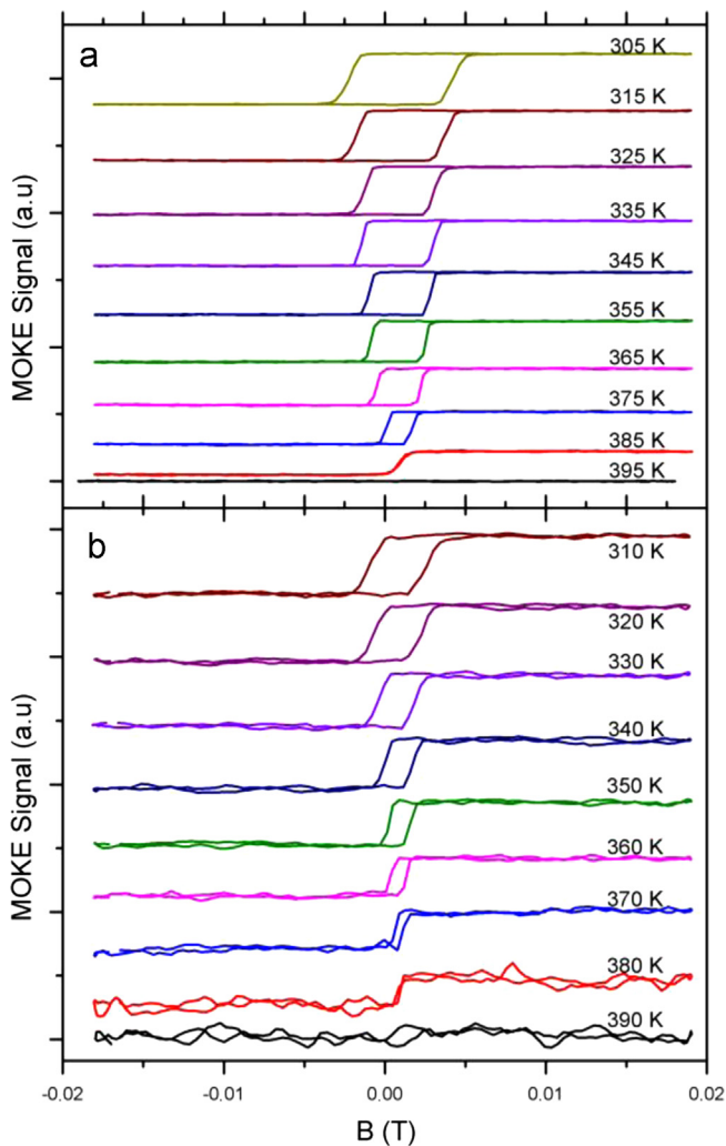
Fig. 1. Temperature-dependent MOKE hysteresis loops of 9.6 ML Ni/Cu 3 Au (001) taken (a) in a longitudinal and (b) in a polar geometry.
