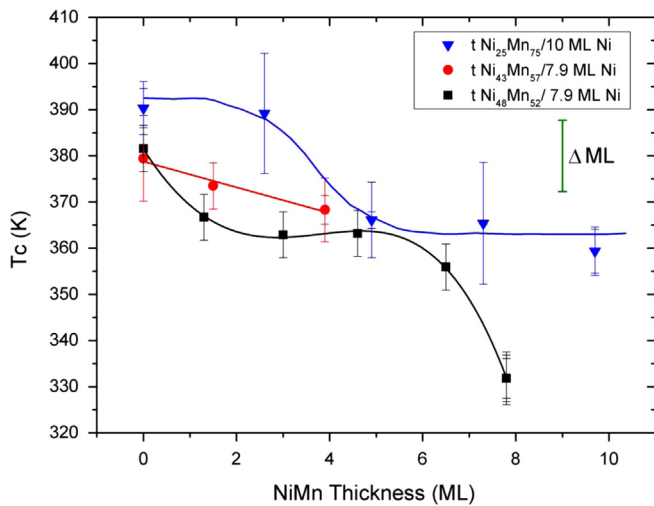
Fig. 5. Ni Curie temperature as a function of the Ni x Mn 1-x thickness for different concentrations in the Mn-rich regime. The scale bar at the right indicates the difference in Curie temperature corresponding to a 1 ML change of the effective Ni thickness estimated from the linear fit in Fig. 2.
