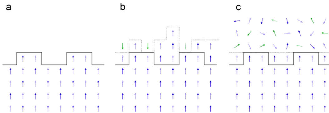
Fig. 4. Schematic model for the Ni Curie temperature changes as a function of the Ni x Mn 1-x thickness in the Ni-rich regime. (a) Ni layer, (b) thin layer of Ni x Mn 1-x on top, and (c) thicker Ni x Mn 1-x layer.
