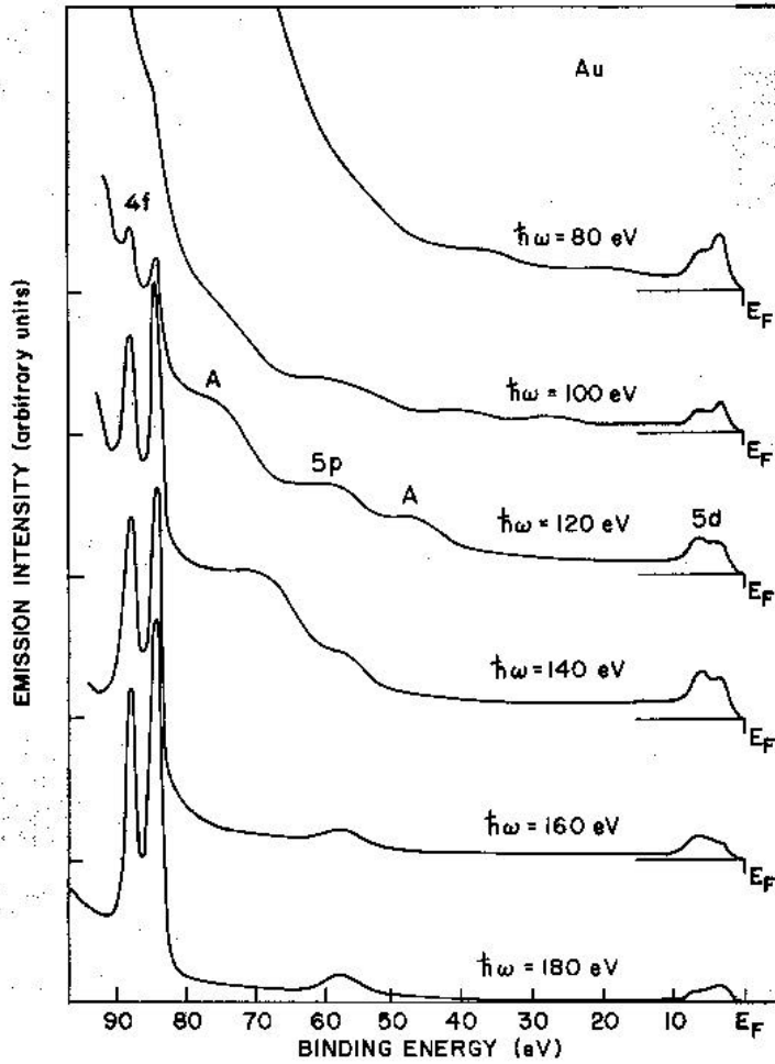
Figure 15. Photoemission spectra of Au for different photon energies between 80 and 180 eV (from Ref. 75).
