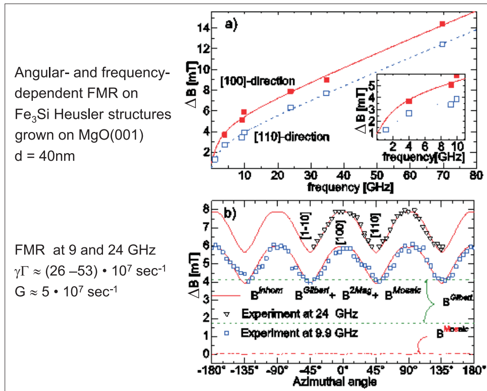
Figure 11. FMR linewidth for Heusler alloys as function of frequency taken from [23]. Note the narrow line at 1 GHz. Figure 11b shows the angular dependent 2-magnon scattering and isotropic Gilbert damping.
