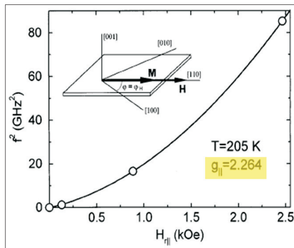
Figure 6. Analysis of g_{\parallel} for \text{Fe}_2\text{V}_5 according to the equation given in figure 4.[14].
