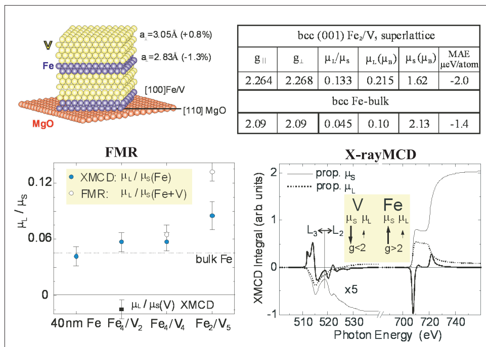
Figure 7. Schematic sketch for epitaxially grown \text{Fe}_n\text{V}_m superlattice structure, FMR and XMCD results, table for g-factors, \mu_L , and \mu_S [7, 14].
