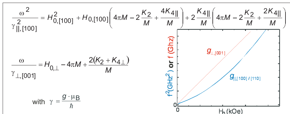
Figure 4. FMR resonance equation for in-plane and out-of plane orientation of the external field H_0 with respect to the crystallographic film plane. For details and notation, see [6, 7].
