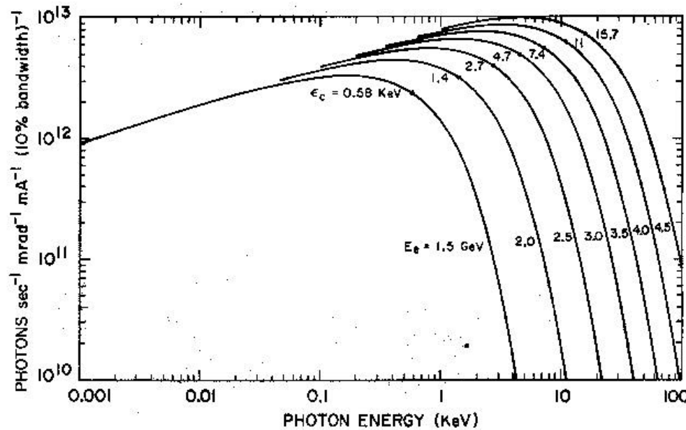
Figure 3. Spectral distribution of synchrotron radiation from SPEAR, ( \rho = 12.7 m).
